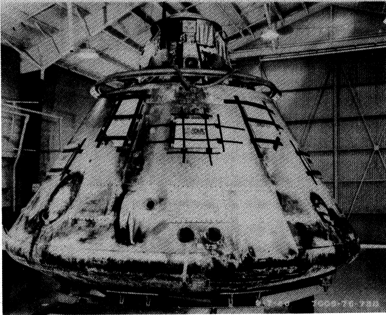
SLIDE 68. SPACECRAFT 011 AFTER RECOVERY
