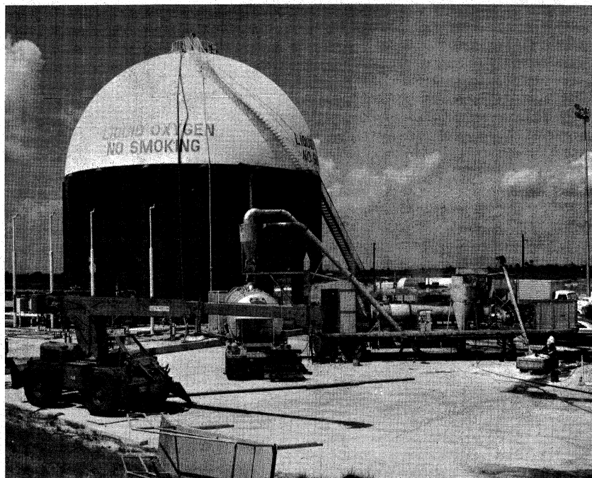
FIGURE D-19.—Liquid oxygen storage tank at launch complex 39, pad A.
