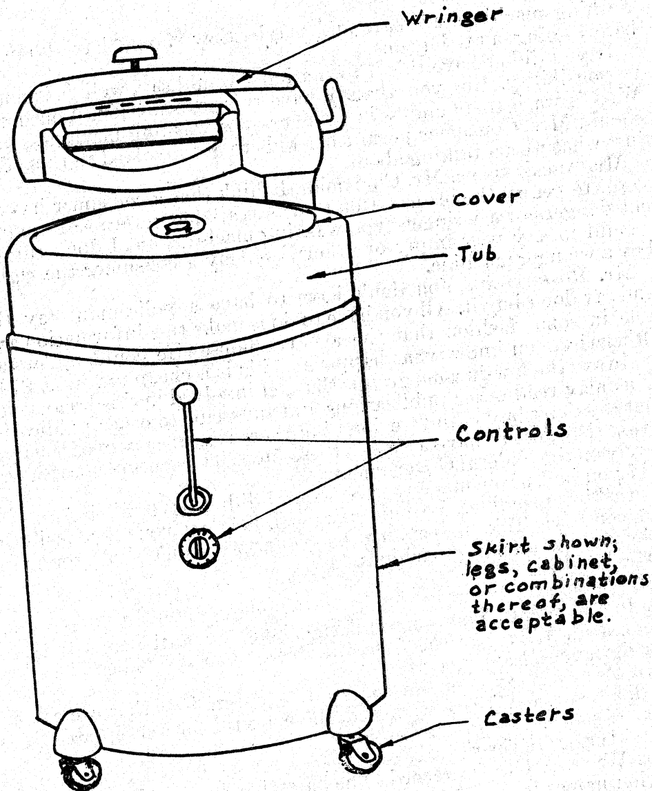
Figure 1. - Type I, class 1 wringer washing machine.
