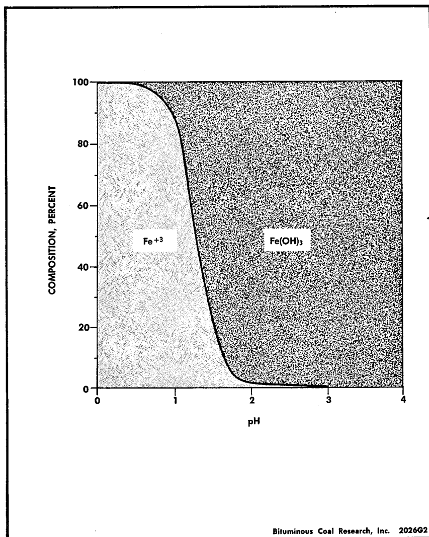
Figure 2. Distribution of \text{Fe}^{+3} and \text{Fe}(\text{OH})_3 as a Function of pH
