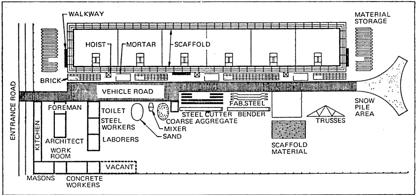
FIG. 1 Example of Winter Building Site Plan
